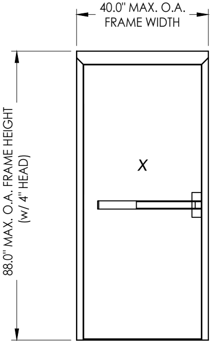
"7700 Series" Fire Exit Device
